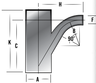
90° TY (STRAIGHT ENDS)
