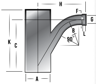
90° TY (ONE END EXPANDED)
