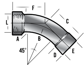
45° FEMALE ADAPTER ELBOW
