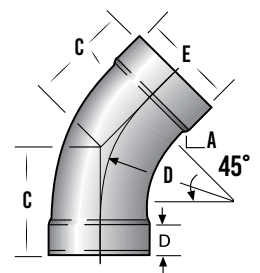
45° SHORT RADIUS ELBOW
