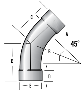
45° STANDARD RADIUS ELBOW
