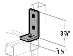
90° STRUT BRACKET 2 HOLES X 1 HOLES
