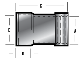
FEMALE REDUCING ADAPTER EXPANDED
