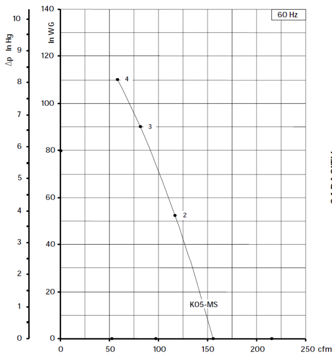
CAPACITY
