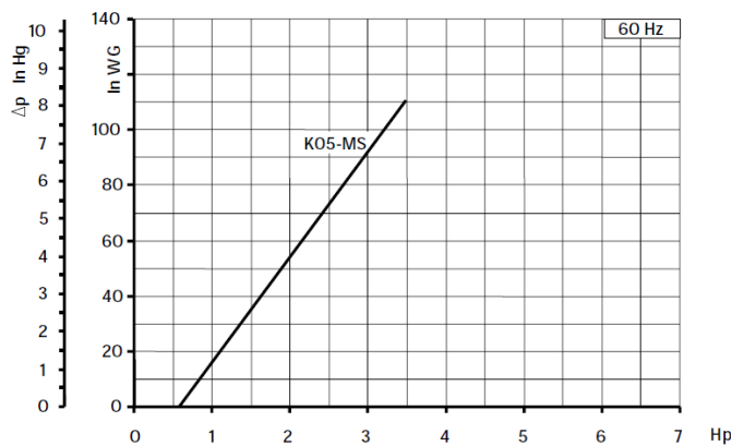
ABSORBED POWER
